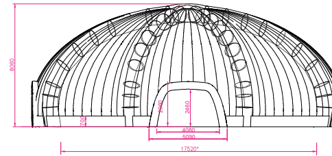
FRONT ELEVATION
