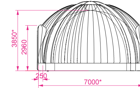
SIDE ELEVATION
