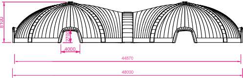
SIDE ELEVATION
